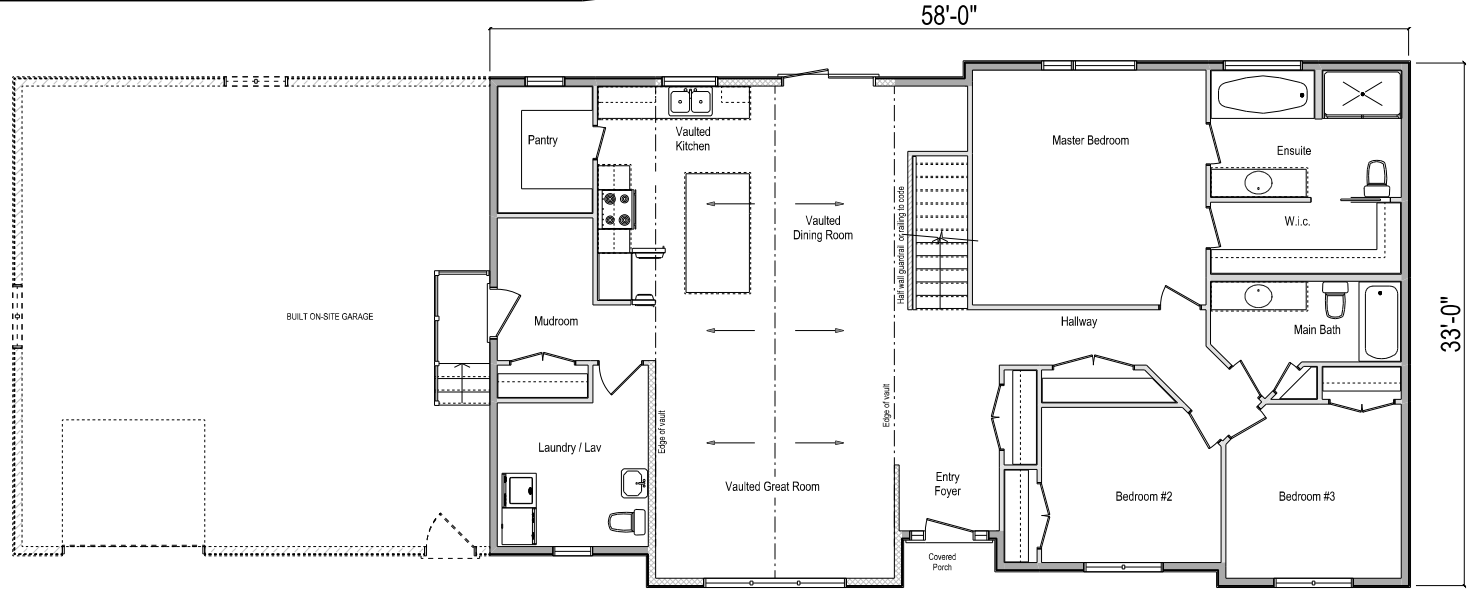
MAIN FLOOR PLAN for a 1832 SF. RTM BUNGALOW Ridgeview Homes READY-TO-MOVE HOME MODEL #2305
