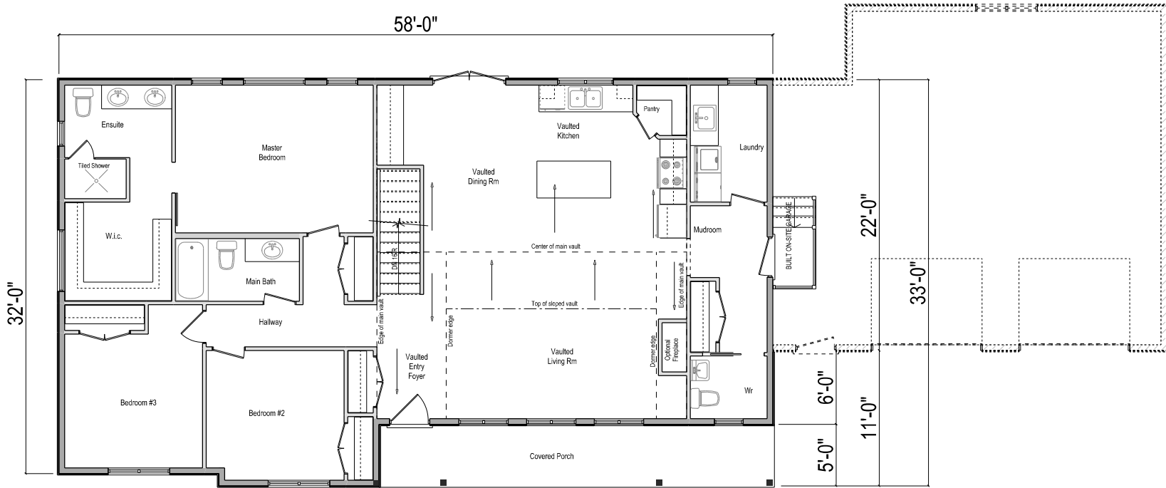
MAIN FLOOR PLAN for a 1741 SF. RTM BUNGALOW
