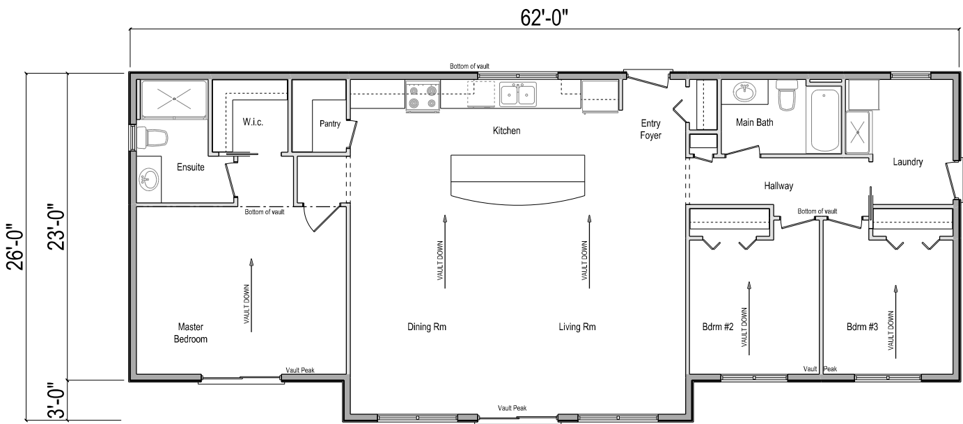
MAIN FLOOR PLAN for a 1504 SF. RTM BUNGALOW
