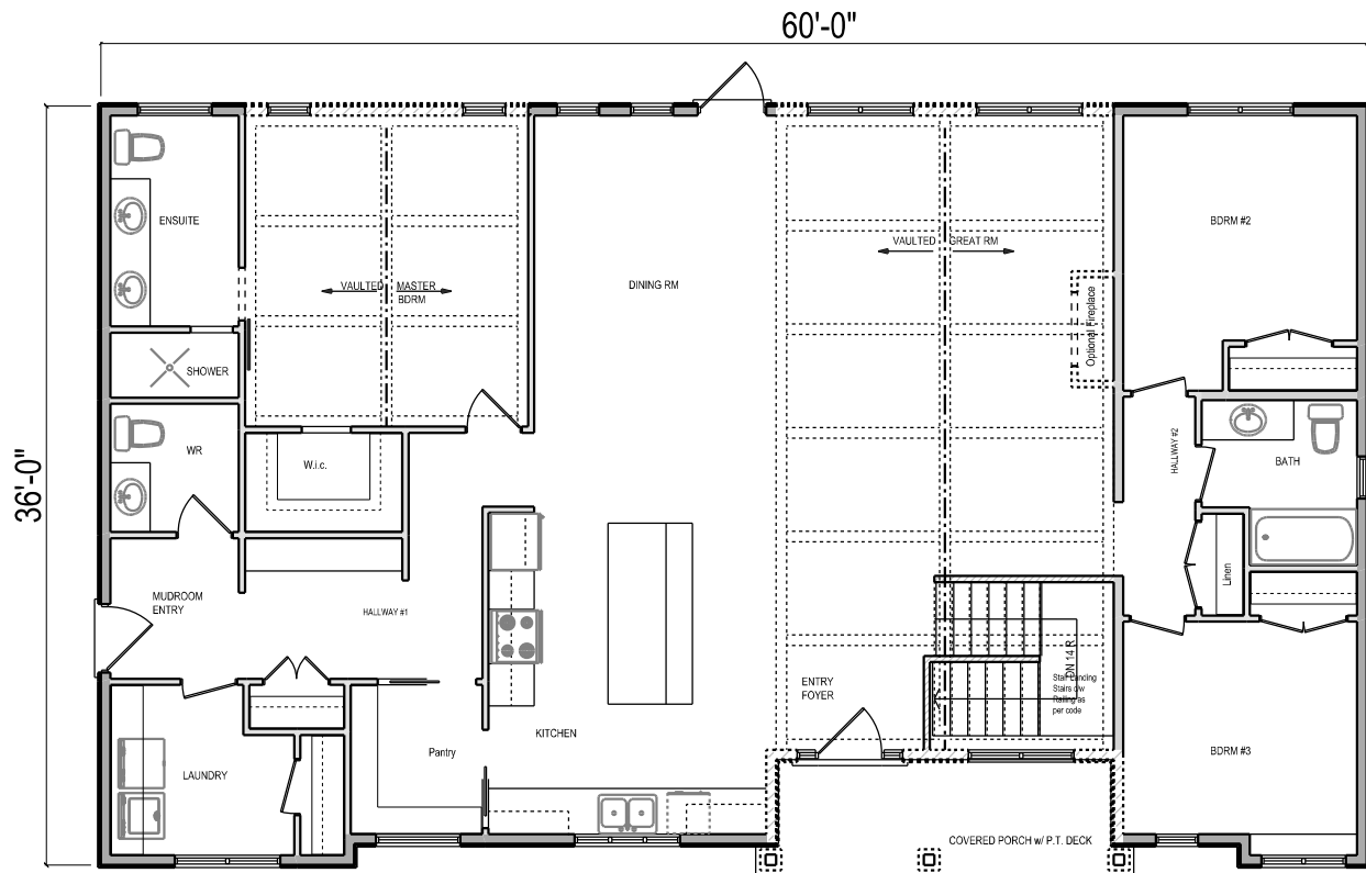
MAIN FLOOR PLAN 2054 SF. RTM BUNGALOW
