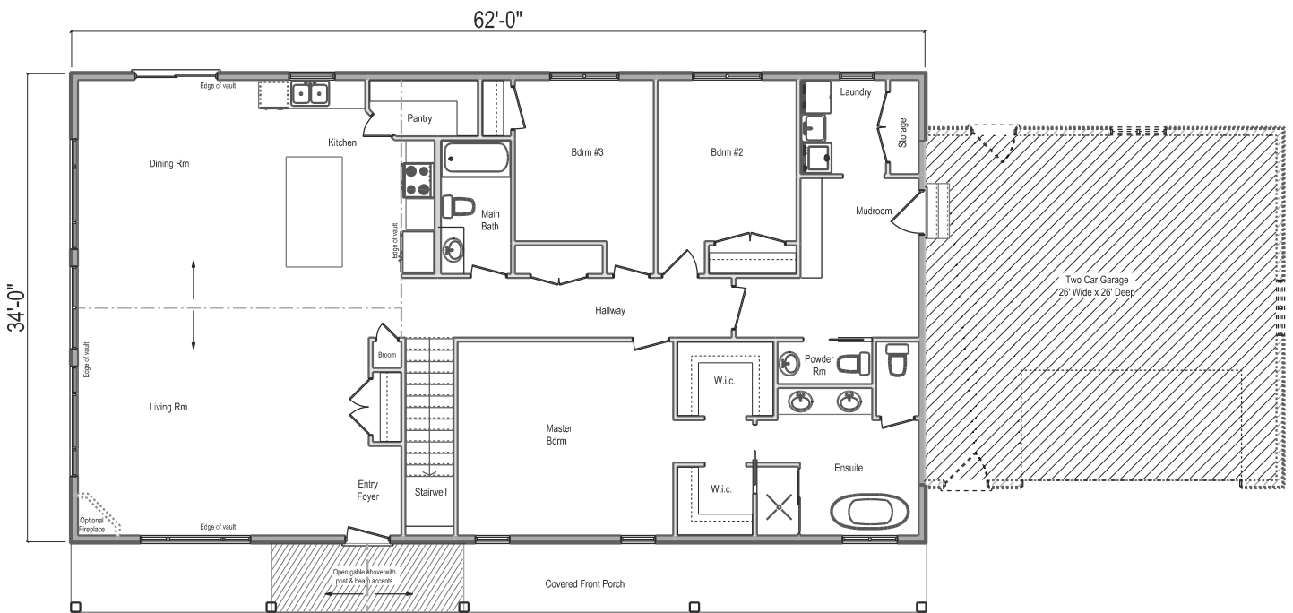
MAIN FLOOR PLAN for a 2108 SF. RTM BUNGALOW
